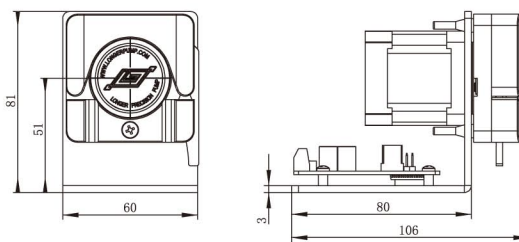
Installation Drawing
