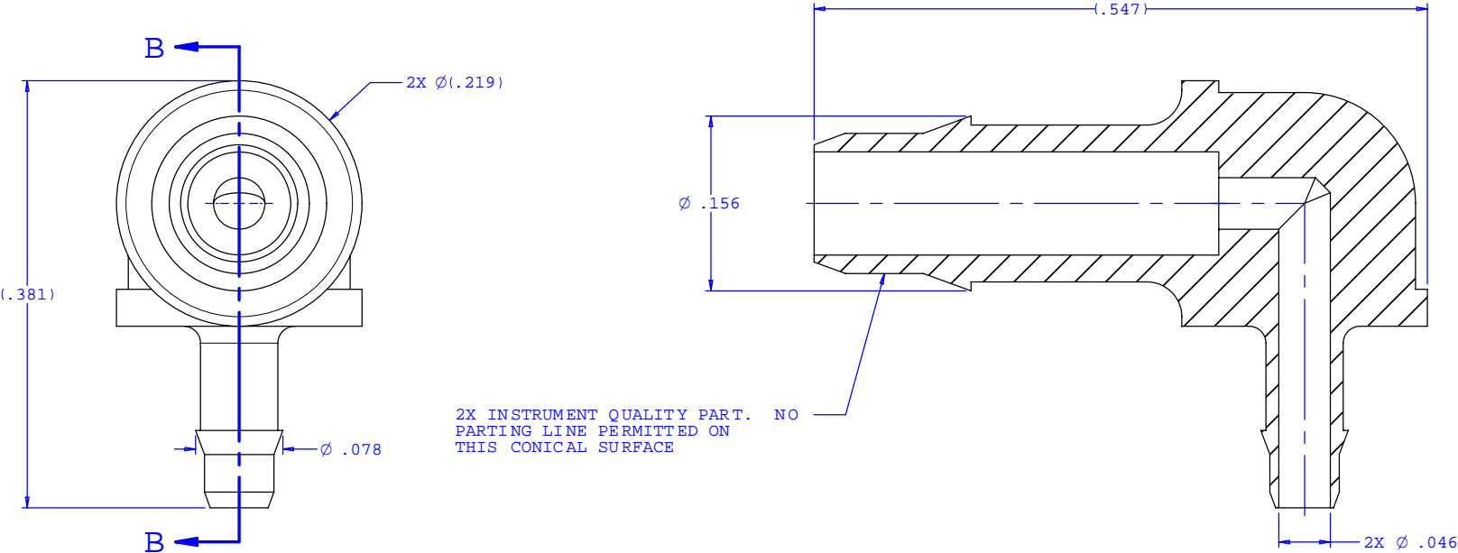
SECTION B-B
